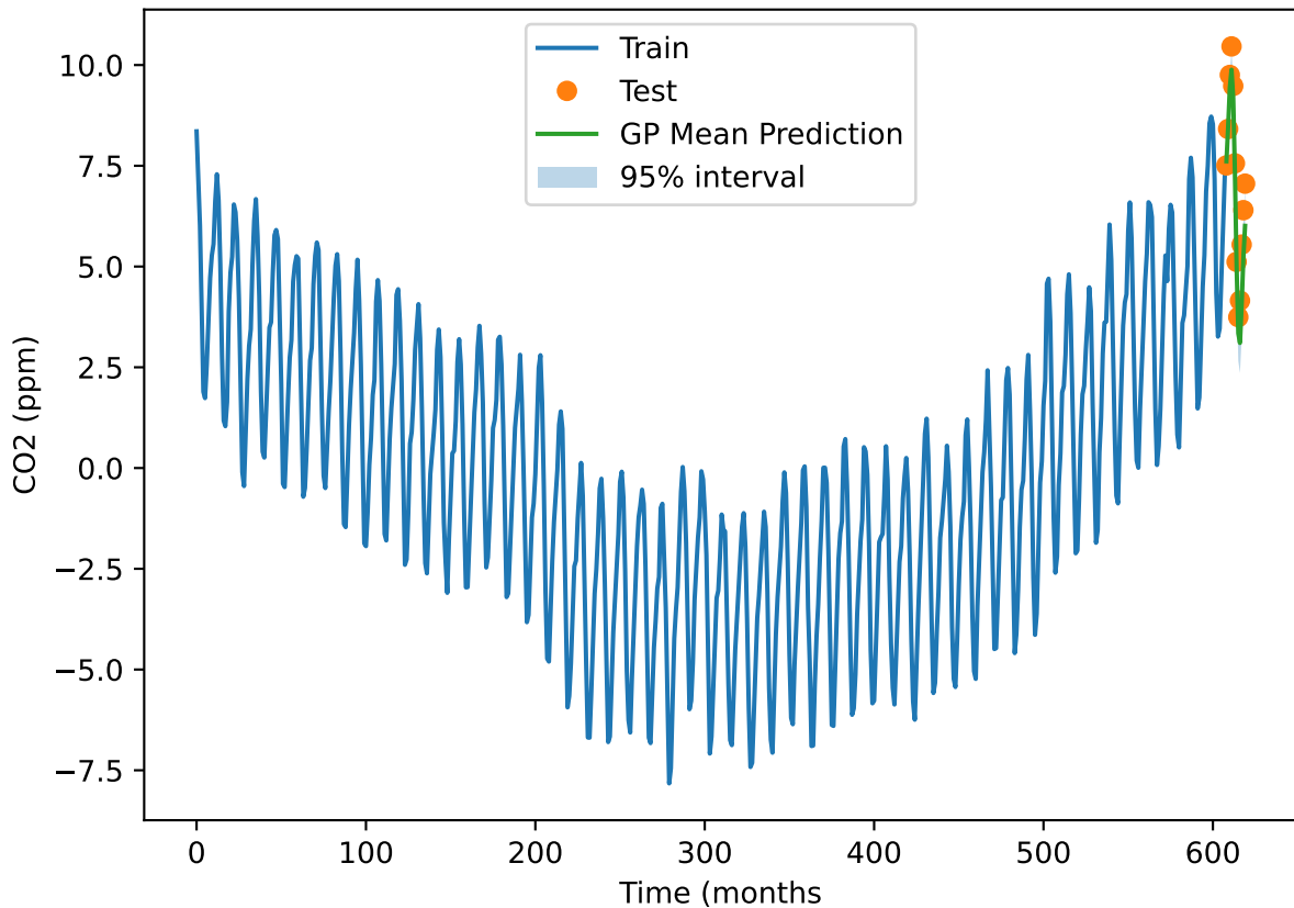
GP Prediction of last 12 months
